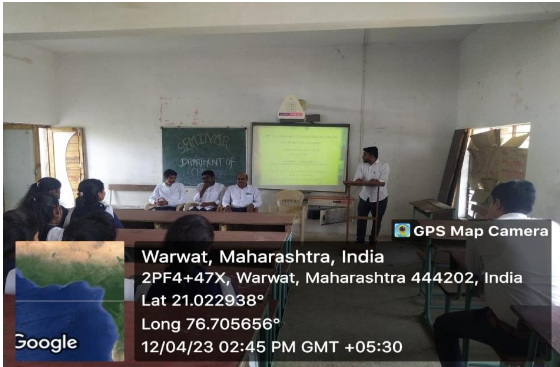
Figure 7- Program Image
